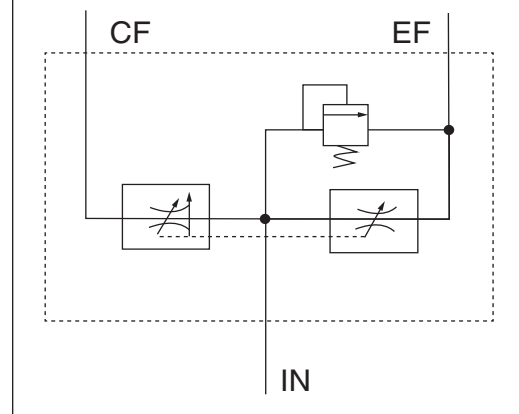
SYMBOLE HYDRAULIQUE HYDRAULIC SYMBOL
